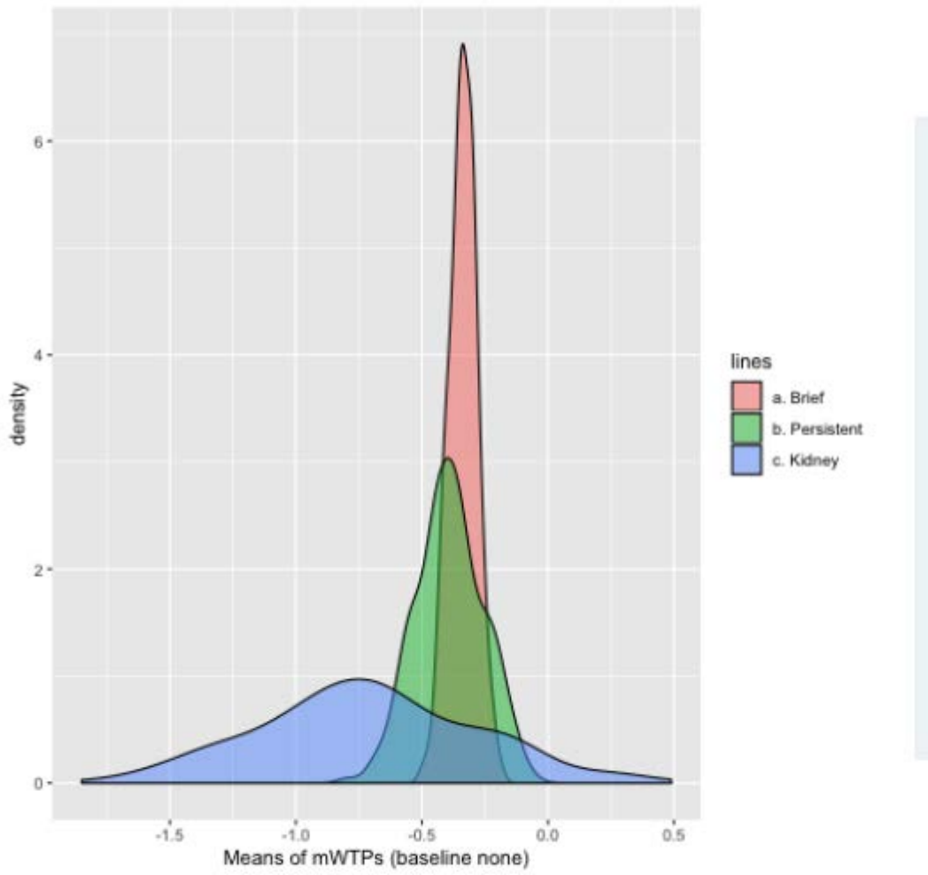
(a) Bayes with correlation, from RStan
