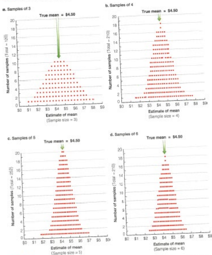
FIGURE 7-7 The Sampling Distributions of Samples of 3, 4, 5, and 6. As we increase the sample size, the possible samples cluster ever more tightly around the true value of the mean. The chance of extremely inaccurate estimates is reduced at the two ends of the distribution, and the percentage of the sample near the true value keeps increasing.
