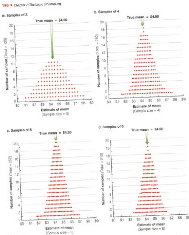
FIGURE 7-7 The Sampling Distributions of Samples of 3, 4, 5, and 6. As we increase the sample size, the possible samples cluster ever more tightly around their true value of the mean. The chance of extremely inaccurate estimates is reduced at the two ends of the distribution, and the percentage of the samples near the true value keeps increasing.
